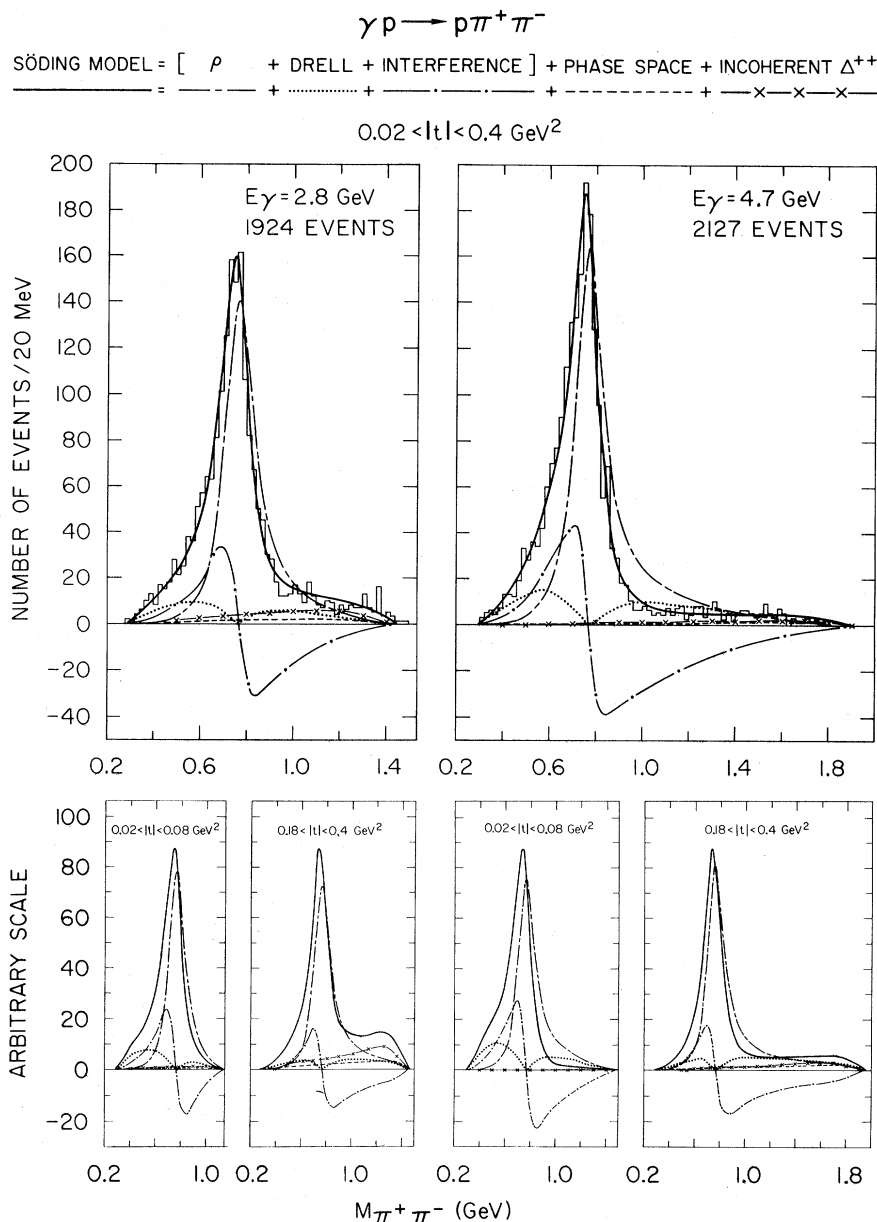
FIG. 30. The contributions of \rho , Drell, interference terms, phase space, and \Delta^{++} to the \pi^+\pi^- mass spectrum from a Söding-model fit to the channel \gamma p \rightarrow p \pi^+ \pi^- in the region 0.02 < |t| < 0.4 \text{ GeV}^2 . The lower diagrams give the contributions in the intervals 0.02 < |t| < 0.08 \text{ GeV}^2 and 0.18 < |t| < 0.4 \text{ GeV}^2 .
