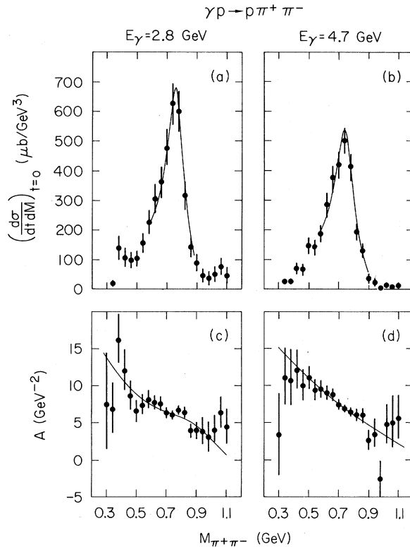
FIG. 11. Reaction \gamma p \rightarrow \rho \pi^+ \pi^- . (a) and (b) d^2\sigma/dt dM|_{t=0} for dipion production obtained from a maximum-likelihood fit of the form Be^{At} to events in the t interval 0.02 < |t| < 0.4 GeV 2 . The solid curve is from a fit of the form Breit-Wigner \times (M_\rho/M_{\pi\pi})^n (see Sec. IV C 3) in the interval 0.6 < M_{\pi\pi} < 0.9 GeV. (c) and (d) The slope, A , of the invariant-momentum-transfer distribution of dipion pairs as a function of dipion mass. The solid curve is from the Söding model (Sec. IV C 2 and Appendix B).
