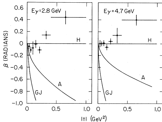
FIG. 17. Reaction \gamma p \rightarrow p \rho^0 . The angle \beta for rotation about the normal to the production plane of the \rho density matrix from the helicity frame into the "minimum-flip" system as a function of t . The curves marked H, A, GJ show where the data points would lie if the minimum-flip system were the helicity, Adair, and Gottfried-Jackson frame, respectively.
