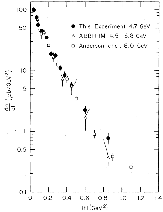
FIG. 25. The differential cross section for \rho^0 production: from this experiment (●) at 4.7 GeV using the parametrization technique; from the ABBHMM collaboration at 4.5–5.8 GeV (Δ) (Ref. 11); from Anderson et al. , (□) at 6 GeV (Ref. 67).
