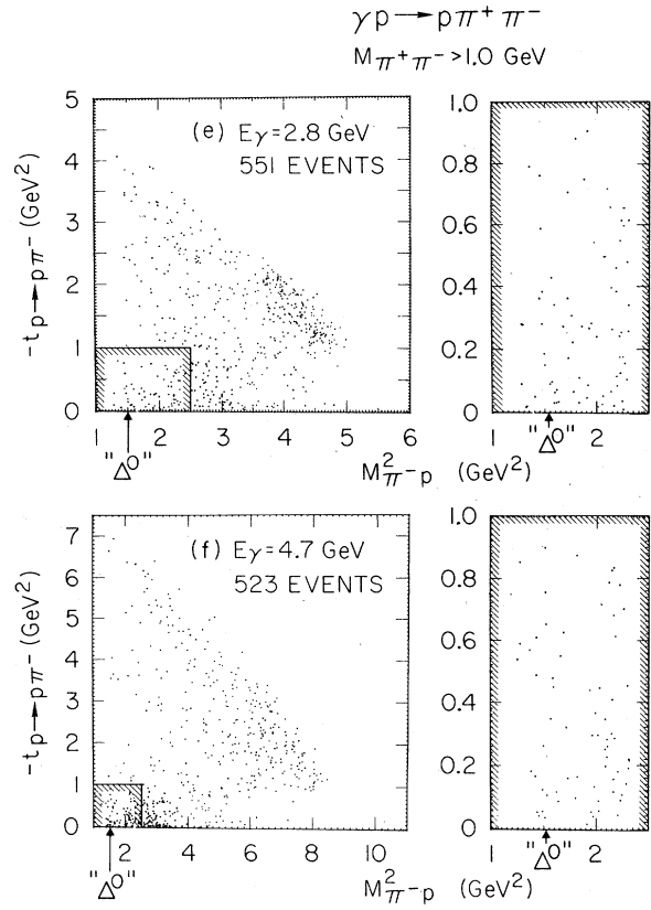
FIG. 9. (a)–(f) Reaction \gamma p \rightarrow p \pi^+ \pi^- . Chew-Low plots for \pi^+ \pi^- , \pi^+ p , and \pi^- p . (c)–(f) are for M_{\pi^+ \pi^-} > 1 GeV. The outlined regions are shown on the right in an expanded scale.
