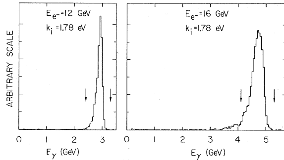
FIG. 2. Photon energy spectra (unnormalized) for the 2.8- and 4.7-GeV runs. The arrows indicate the energy intervals used. The ordinate gives the number of photons.
