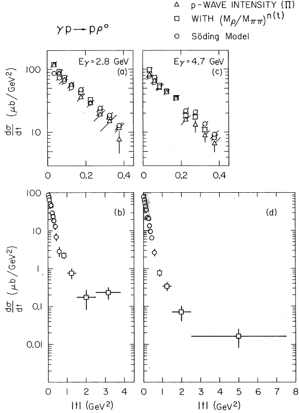
FIG. 19. Reaction \gamma p \rightarrow p \rho^0 . Differential cross sections as a function of t for the helicity-conserving p -wave contribution \Pi(\Delta) , for \rho^0 production as obtained from fits with the Söding model ( \circ ) and from the parametrization (M_\rho/M_{\pi\pi})^{n(t)} ( \square ). The shaded regions are shown above on an expanded scale.
