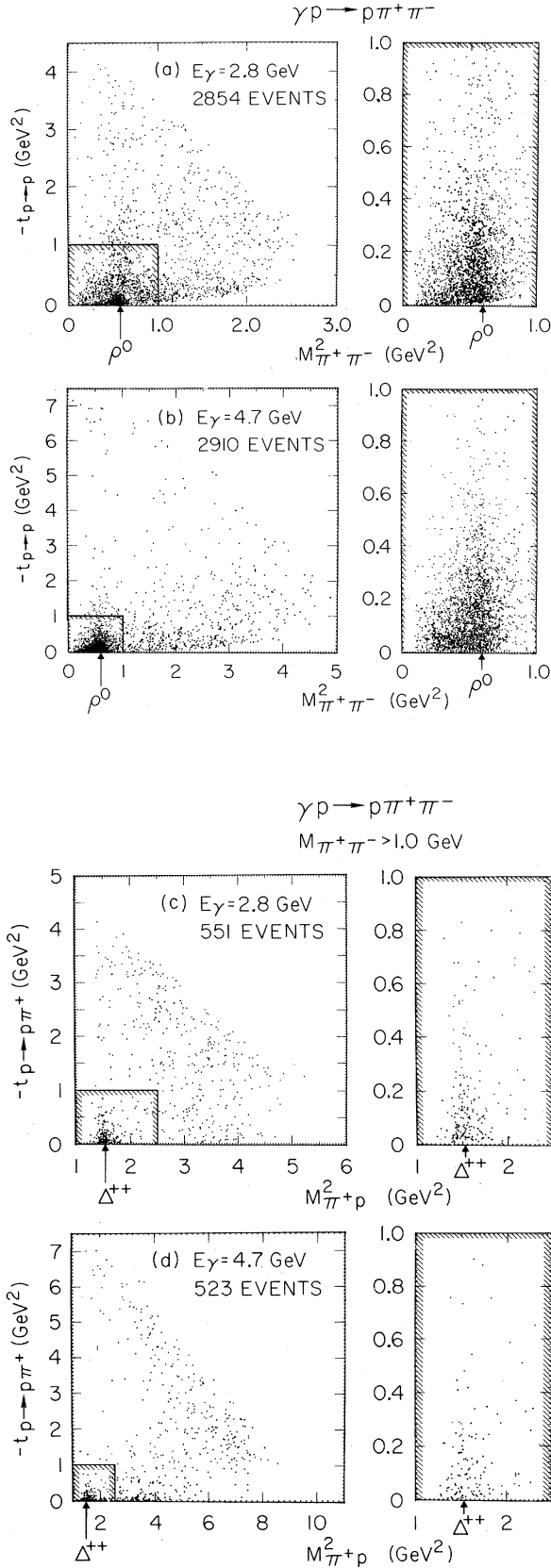
FIG. 9. (a)–(f) Reaction \gamma p \rightarrow p \pi^+ \pi^- . Chew-Low plots for \pi^+ \pi^- , \pi^+ p , and \pi^- p . (c)–(f) are for M_{\pi^+ \pi^-} > 1 GeV. The outlined regions are shown on the right in an expanded scale.
