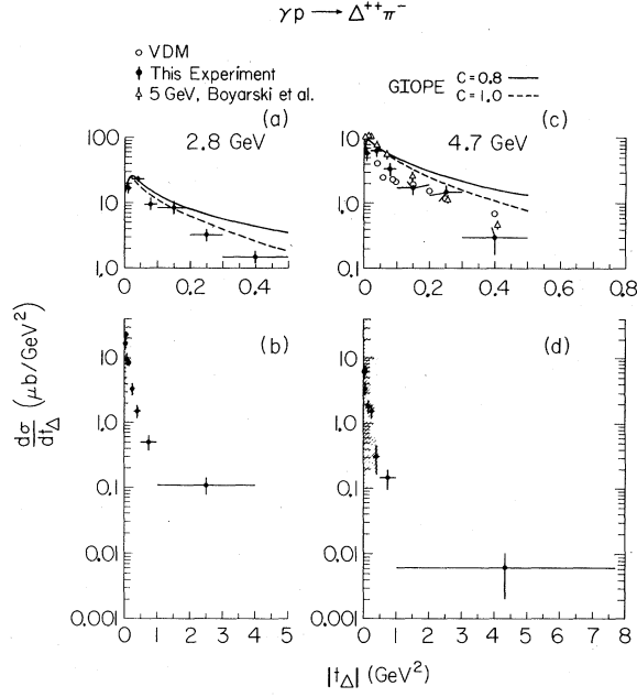
FIG. 27. Reaction \gamma p \rightarrow \Delta^{++} \pi^- . Differential cross sections d\sigma/dt_\Delta from this experiment ( \bullet ) and from Ref. 73 for E_\gamma = 5 GeV ( \Delta ). The shaded regions in (b) and (d) are shown on an expanded scale in (a) and (c). The curves are the predictions of the gauge-invariant OPE model with absorption corrections for C = 0.8 (solid line) and C = 1 (dashed line). The points (O) are the VDM prediction of Ref. 82.
