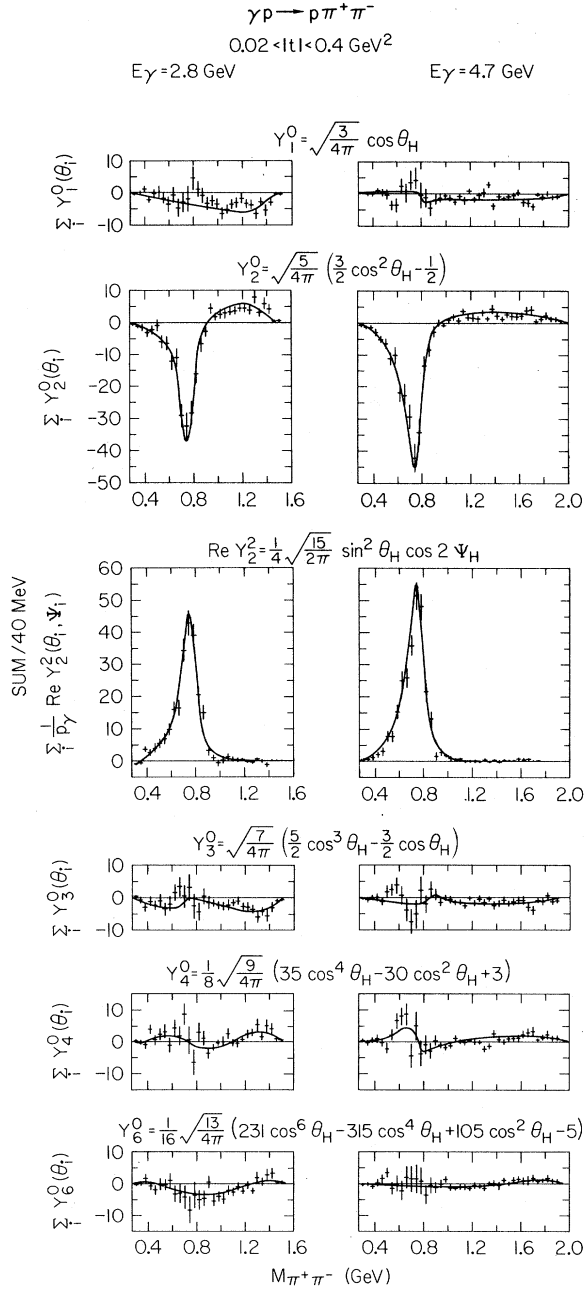
FIG. 14. Reaction \gamma p \rightarrow p \pi^+ \pi^- . The dipion moments Y_1^0(\theta) , Y_2^0(\theta) , \text{Re } Y_2^2(\theta, \Psi) , Y_3^0(\theta) , Y_4^0(\theta) , Y_6^0(\theta) in the helicity frame as a function of M_{\pi^+ \pi^-} for 0.02 < |t| < 0.4 \text{ GeV}^2 . The curves are obtained from the Söding model (Sec. IV C 2).
