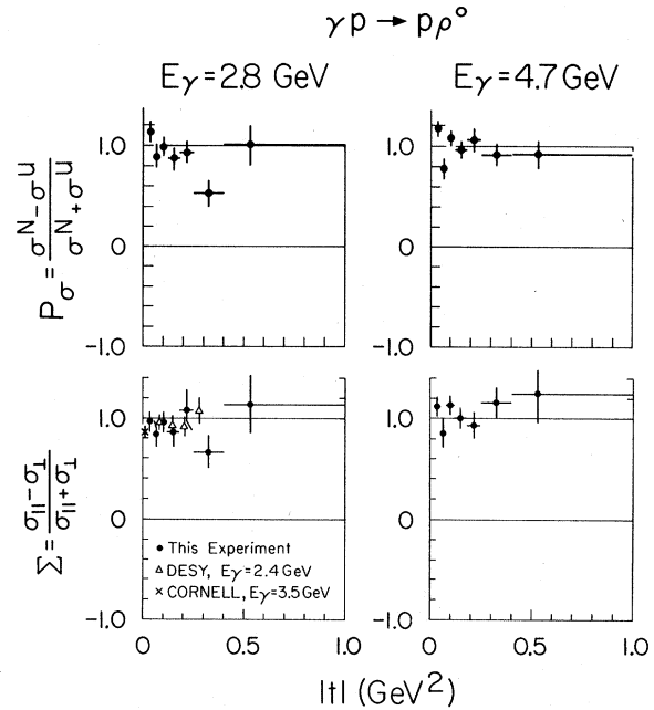
FIG. 18. Reaction \gamma p \rightarrow p \rho^0 . The parity asymmetry, P_0 , and the asymmetry, \Sigma , as a function of t . The points labeled DESY and Cornell are from Refs. 40 and 41, respectively.
